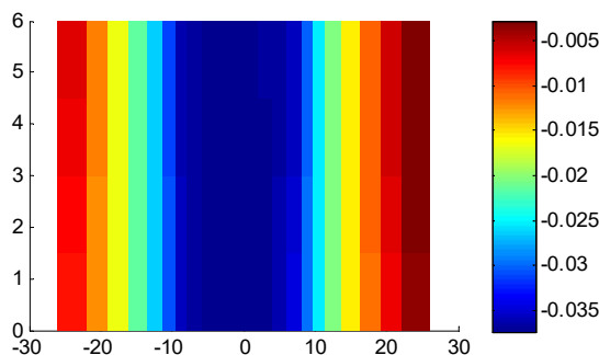
Fig. 11 Vertical deformation contour at the ground surface after 6 m completion drilling
