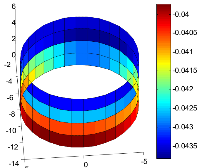
Fig. 12 Vertical deformation contour in the tunnel wall after 6 m completion drilling
